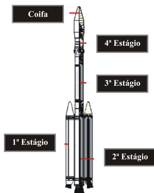
Figura 2: VLS-1 (AEB, 2007).
