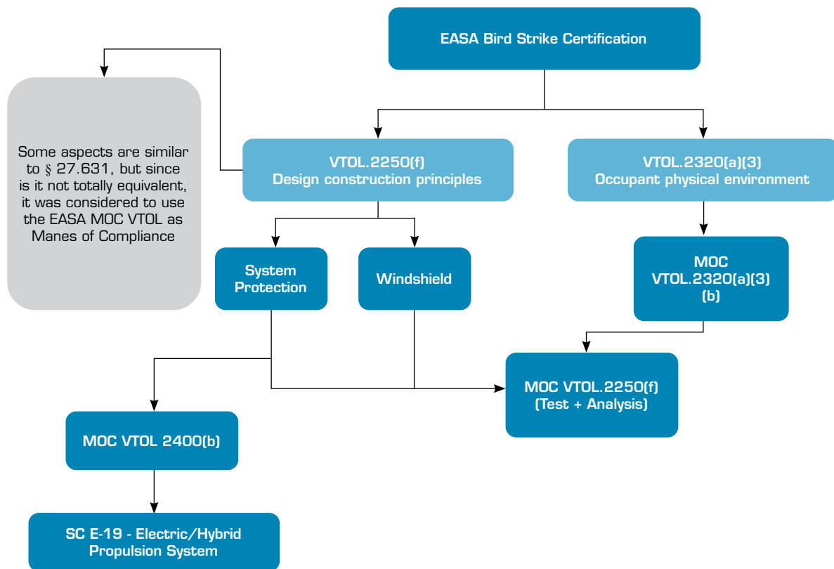
Figure 6. EASA bird strike certification.
