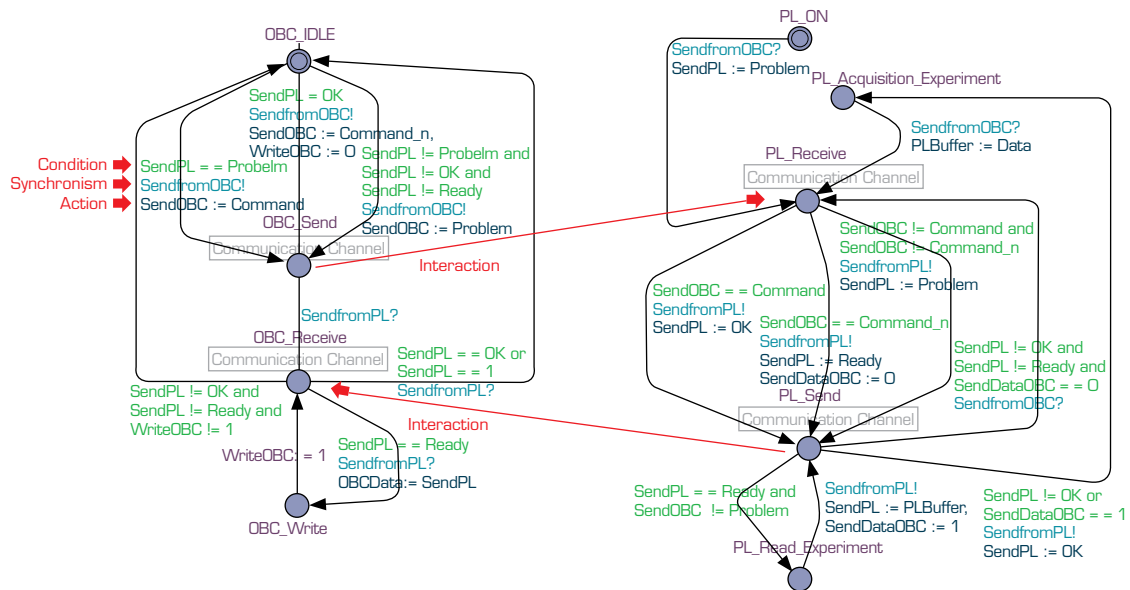
Figure 7. Modeling of OBC and PL subsystems in interaction.
