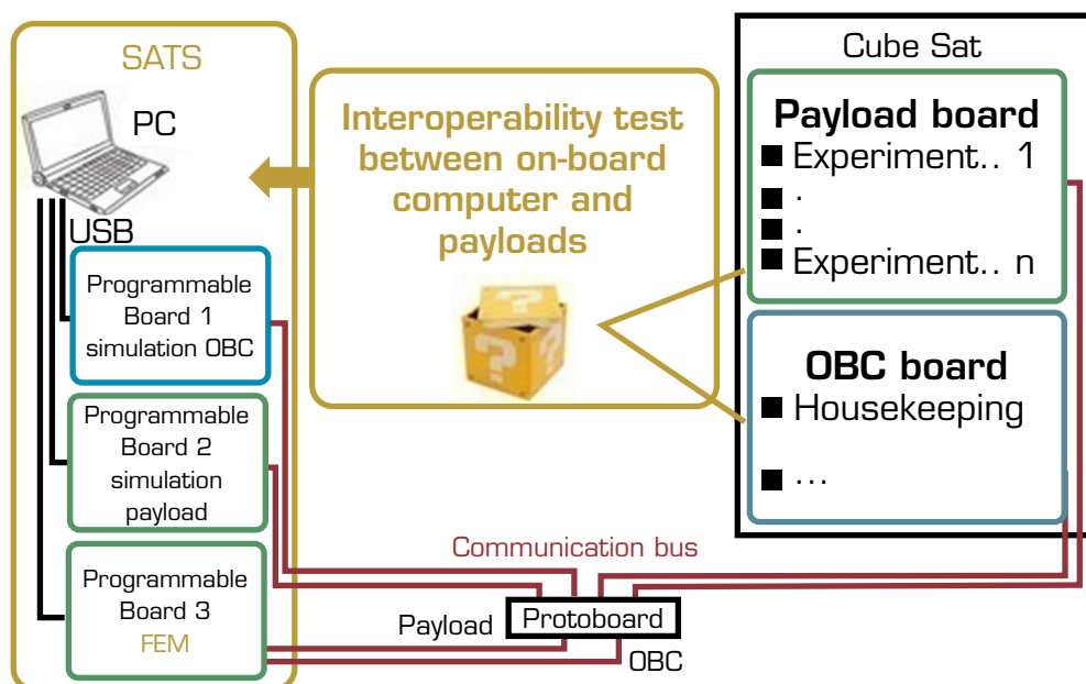
Figure 3. Test architecture with SATS.
