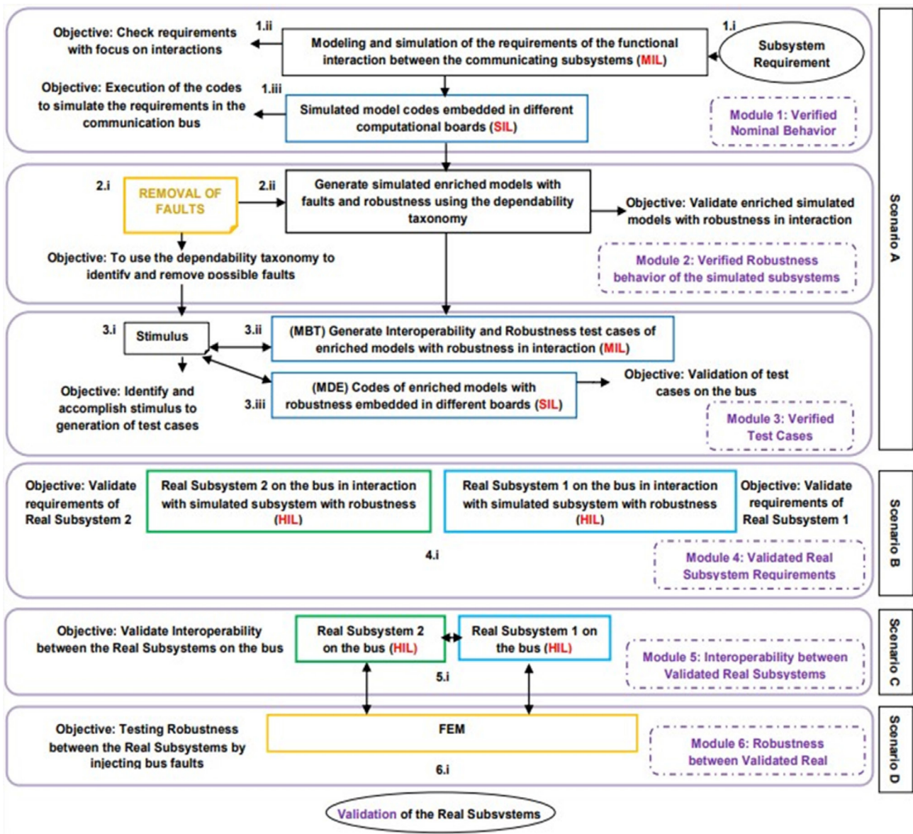
Figure 2. Systematic testing in six modules.
