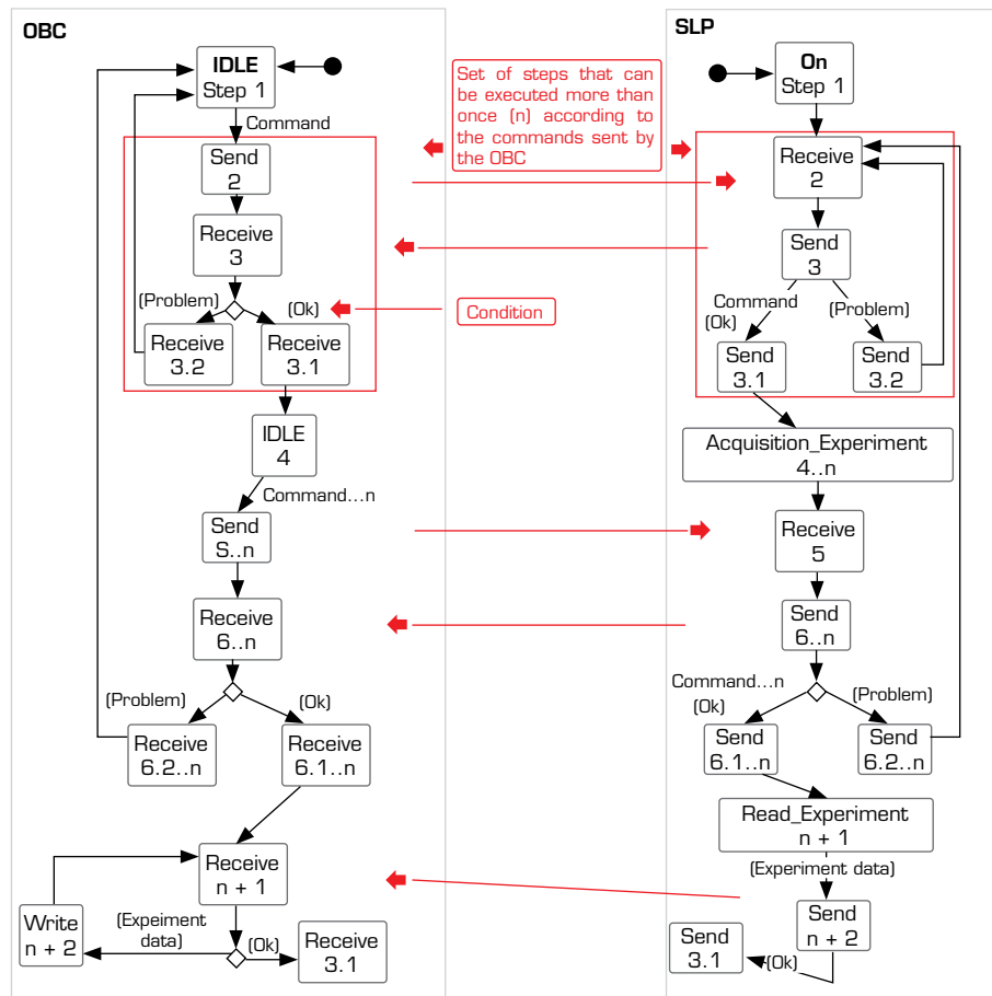
Figure 6. Activity diagram of interoperability between OBC and SLP.
