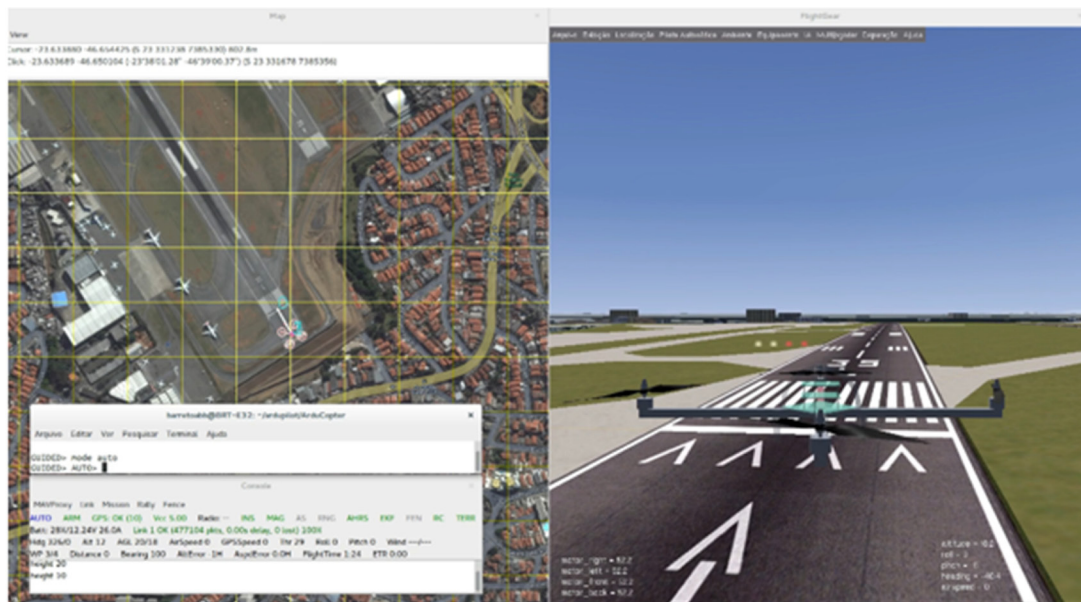
Figure 8. Unmanned aerial systems (UAS)-based PAPI inspection simulator interface.
