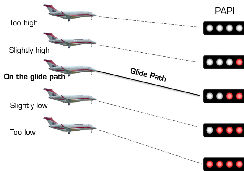
Figure 3. Precision approach path indicator (PAPI) light configuration indicating correct descent rate.
