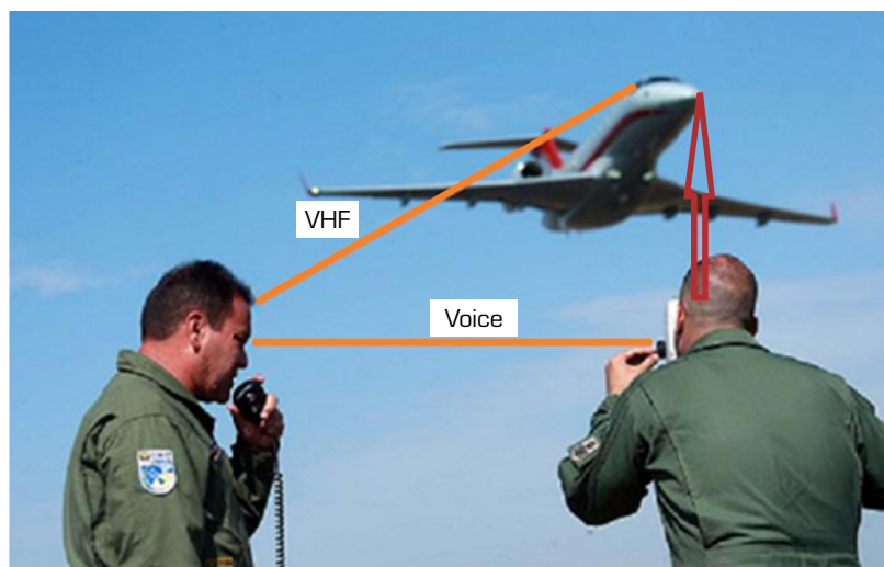
Figure 4. Theodolite-based PAPI inspection method, where the ground operator aligns the theodolite with the aircraft's nose (radome), while a team member communicates with the flight crew via VHF radio for coordination.
