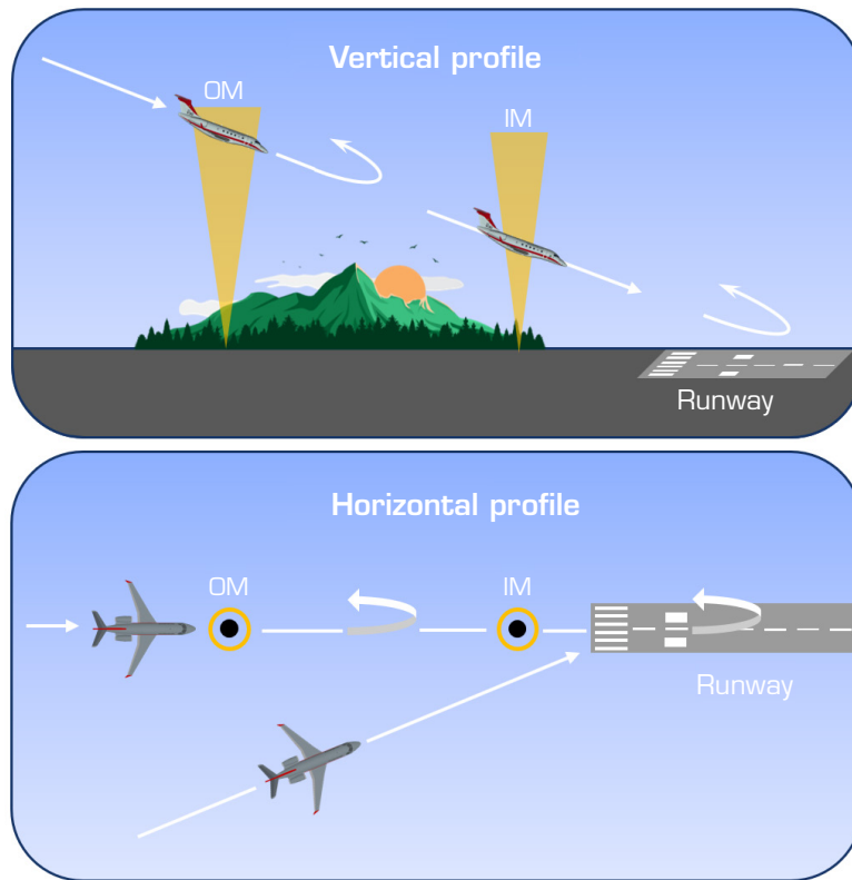
Figure 6. Pattern 3 run profile with go-around maneuvers. IM = inner marker.
