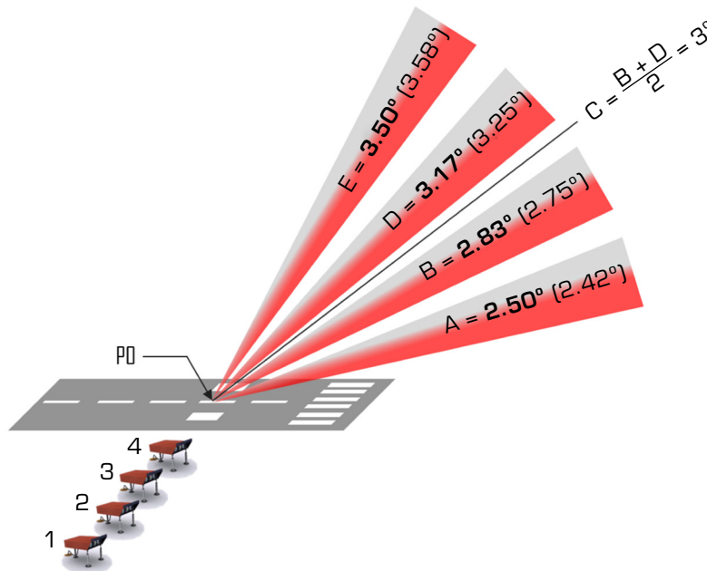
Figure 2. Precision approach path indicator (PAPI) light arrangement for a 3° approach path. The identified angles from the PO are the following: A: low transition; B: medium-low transition; C: nominal ramp; D: medium-high transition angle; and E: high transition. Angles in parentheses are standard values for ILS-connected installation and for large aircraft.
