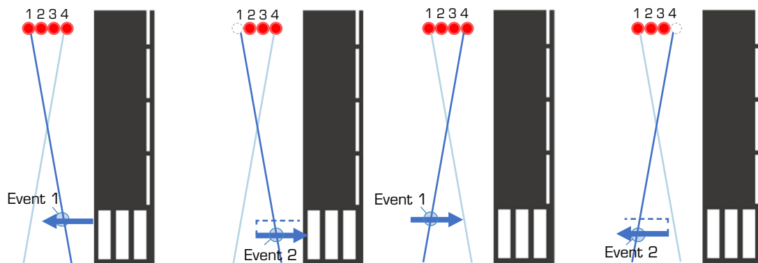
Figure 13. Events of incremental horizontal scanning: instant when all lights are turned on (Event 1) and first light is switched off (Event 2).
