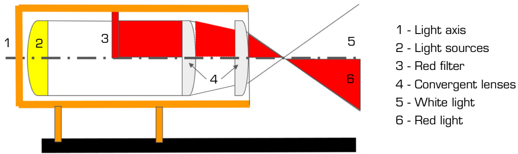
Figure 1. Components of a PAPI light box.
