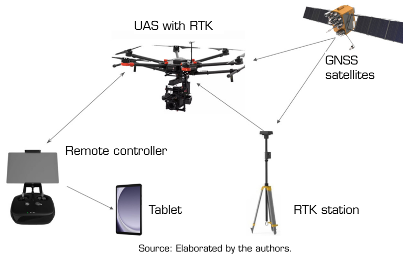
Figure 15. Real-time kinematic (RTK) positioning system used for precise geolocation.
