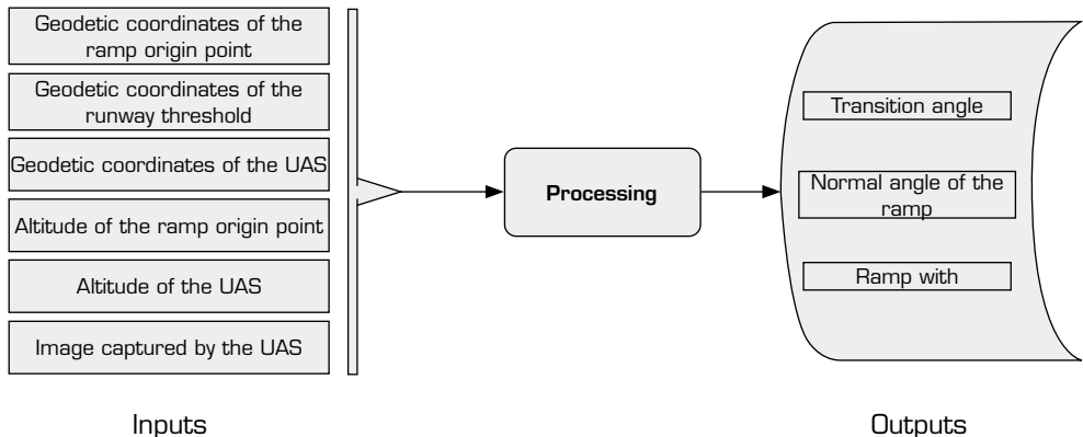
Figure 17. Horizontal scanning processing diagram.
