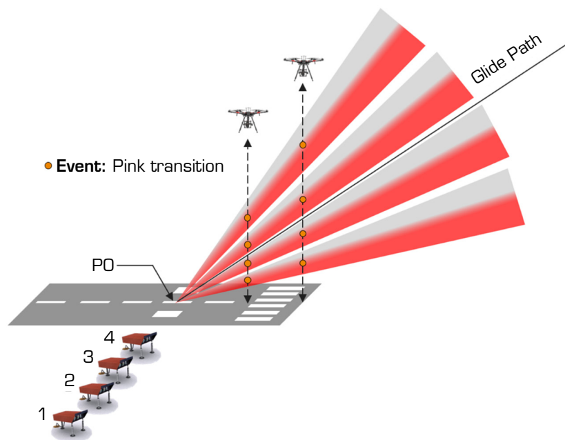
Figure 9. Vertical scanning method for descent angle verification.
