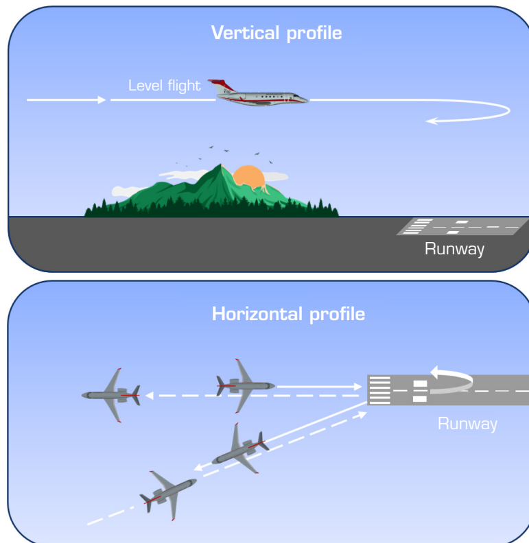
Figure 5. Flight profile Pattern 2 for vertical inspection.
