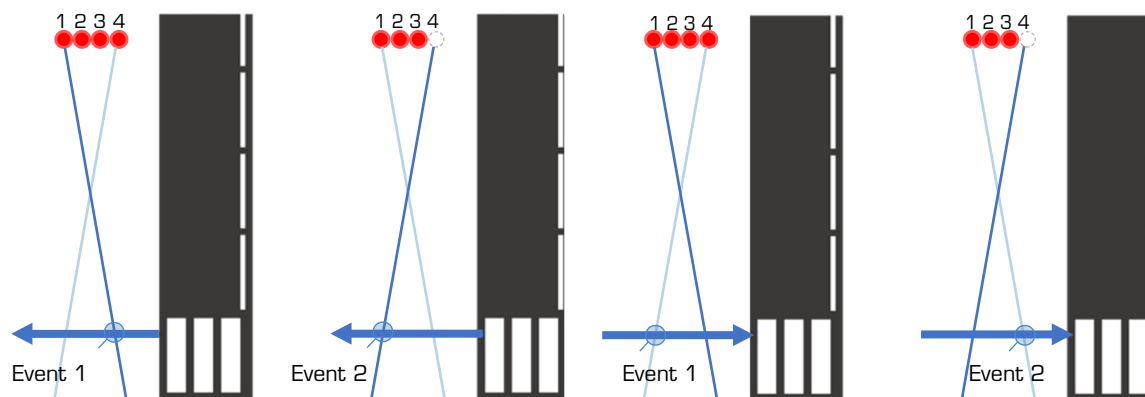
Figure 11. Events of incremental horizontal scanning: instant when all lights are turned on (Event 1) and first light is switched off (Event 2).
