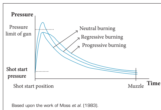
Figure 2. Pressure-time curves for different burning rates.
