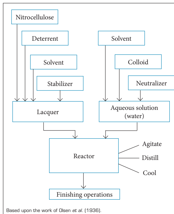
Figure 1. Spherical powder manufacturing process.
