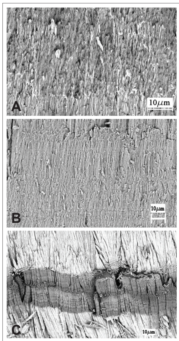
Figure 2: SEM of EB-PVD ceramic coatings fractured cross-section. (A) Sample 1 (column diameter=1.15 μm), (B) Sample 6 (column diameter=1.29 μm), (C) Sample 11 (column diameter=2.53 μm).
