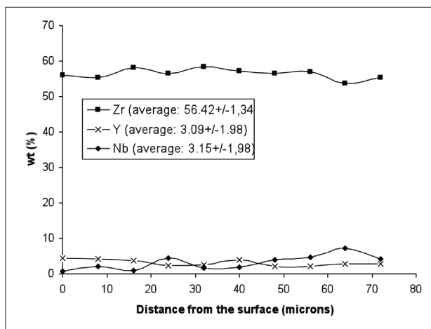
Figure 5: EDS semi-quantitative analysis of ceramic layer (sample 11).
