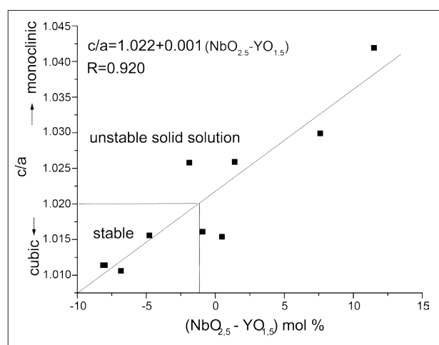
Figure 3: Relation between difference ( \text{NbO}_{2.5} - \text{YO}_{1.5} ) mol% and tetragonality ( c/a ).
