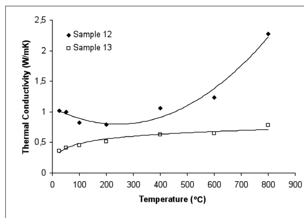
Figure 6: Variations of coatings thermal conductivity with temperature.
