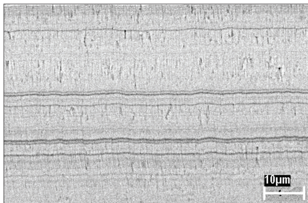
Figure 4: SEM (BS mode) of an EB-PVD ceramic coating polished cross-section (sample 3).
