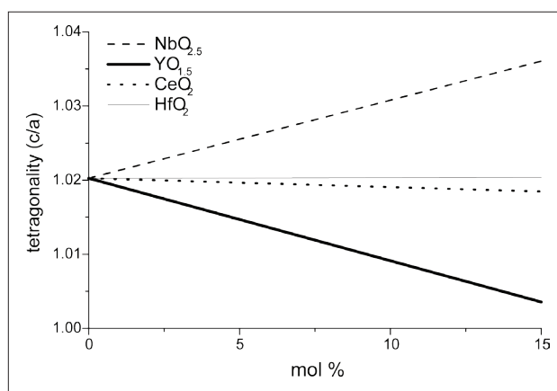
Figure 1: Influence of the alloying oxide in the c/a axial ratio of bulk zirconia-based ceramics.
