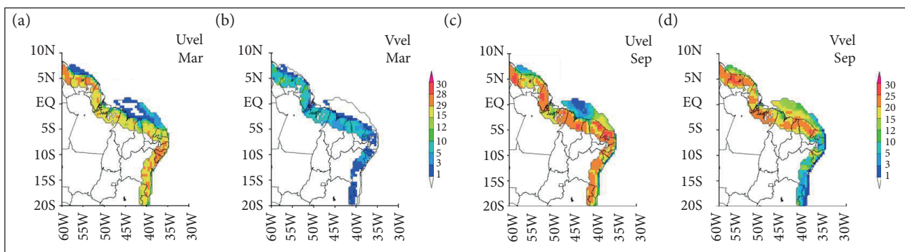
Figure 9. The average breeze potential frequency (number of days per month) in March (a and b) and September (c and d) for the areas shaded in Fig. 3. The left-side panels (a and c) refer to the climatology obtained using the zonal wind data (Uvel); the right-side panels (b and d) refer to the climatology obtained using the meridional wind data (Vvel).
