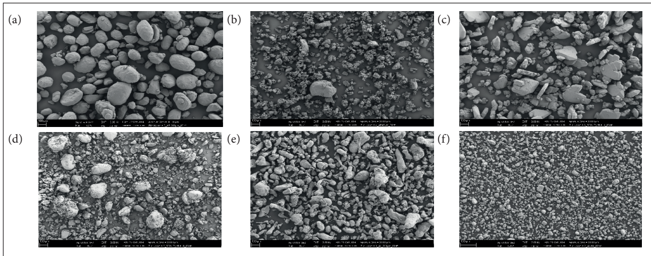
Figure 7. SEM images (magnification of 50X) of the particles loaded in the CSP in this study. (a) Coarse AP, rounded; (b) Fine AP, non-rounded [AP] particles; (c) Coarse RDX, non-rounded; (d) Fine RDX, rounded; (e) Coarse Al, rounded; (f) Fine Al, rounded. Scale of 100 \mu\text{m} .
