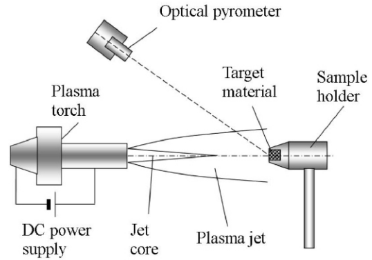
Figure 6: Schematic illustration of the apparatus for ablative test using an arc plasma torch
