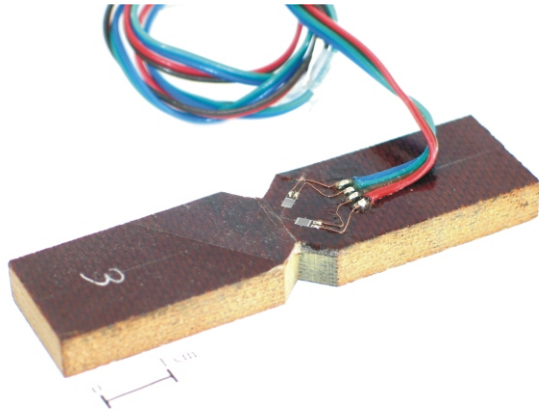
Figure 4: Sample of silica fabric with strain-gages
