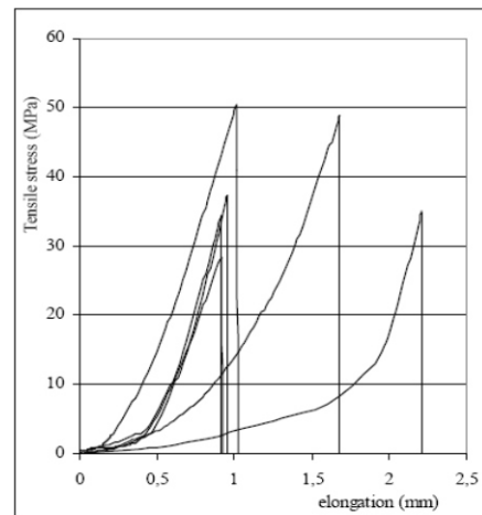
Figure 7: Tensile stress for as cured samples
