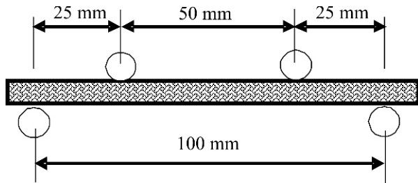
Figure 5: Sample geometry for flexural test Ablative test
