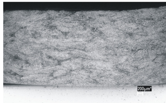
Figura 15: Side view of the specimen before exposure to the plasma torch
