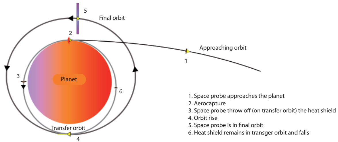
Figure 12. Aerocapture (Stanek 1992).
